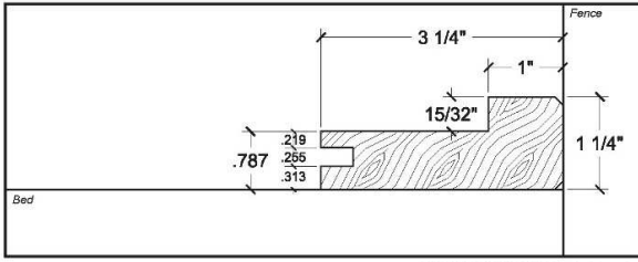
HEAD CONFIGURATION (in feed position)
